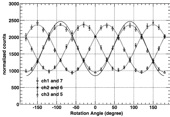
Fig. 6. Normalized counts in peripheral scintillators as a function of rotation angle for 73 keV run. Best fit models are given as dotted lines. For channels 3 and 5, the prediction by Geant4 (with modifications; see text) for the 100% linearly polarized beam is shown by a thin solid line.
