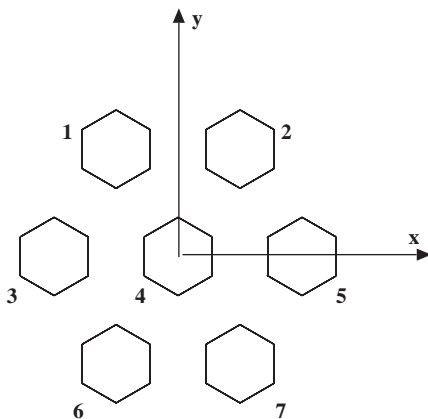
Fig. 2. The layout and numbering scheme of scintillators viewed from the beam origin. Detector rotation angle is defined to be 0^\circ when scintillators channels 3, 4 and 5 are along the horizontal ( x -axis), and to be 30^\circ when channels 1, 4 and 7 are along the vertical ( y -axis).
