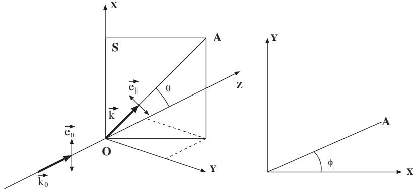
Fig. A2. A photon scattering at point O. The momentum vector ( \vec{k}_0 ) and the polarization vector ( \vec{e}_0 ) of an incident photon are along the z- and x-axis, respectively. \theta and \phi are the scattering polar and azimuth angle. Plane S is constructed by \vec{e}_0 and \vec{k} , the momentum vector after the scattering. \vec{e}_{\parallel} is in plane S.
