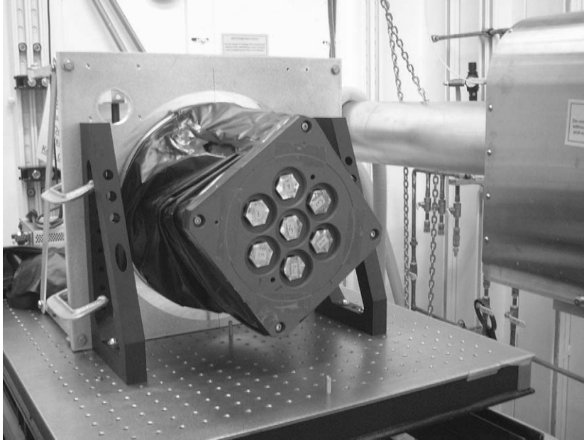
Fig. 3. A photograph of the PoGO prototype mounted on the rotation stage attached to the experiment table.
