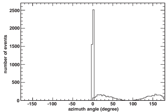
Fig. A1. Azimuthal angle distribution of the polarization vector of 100% linearly polarized photons, after the first Compton scattering. Beam energy is 100 keV and forward scattering events ( \cos \theta \geq 0.95 ) are selected. Distribution obtained by original Geant4 codes is given by a thin solid line and that with our fixes by a thick one. The vector is parallel to the initial beam polarization vector when the angle is 0^\circ .
