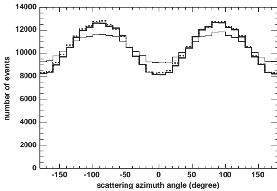
Fig. A4. Predicted azimuthal angle distribution of the Crab Nebula spectrum observed by the PoGO instrument. Like for Fig. A3, the predictions by modified Geant4, original Geant4 and EGS4 are shown by a thick solid line, a thin solid one and a dotted line, respectively.
