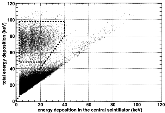
Fig. 5. Relation of deposit energy in the central scintillator and total energy deposition for 73 keV run at 0°. Event selection criteria used in data analysis are also shown by dotted lines (see text).
