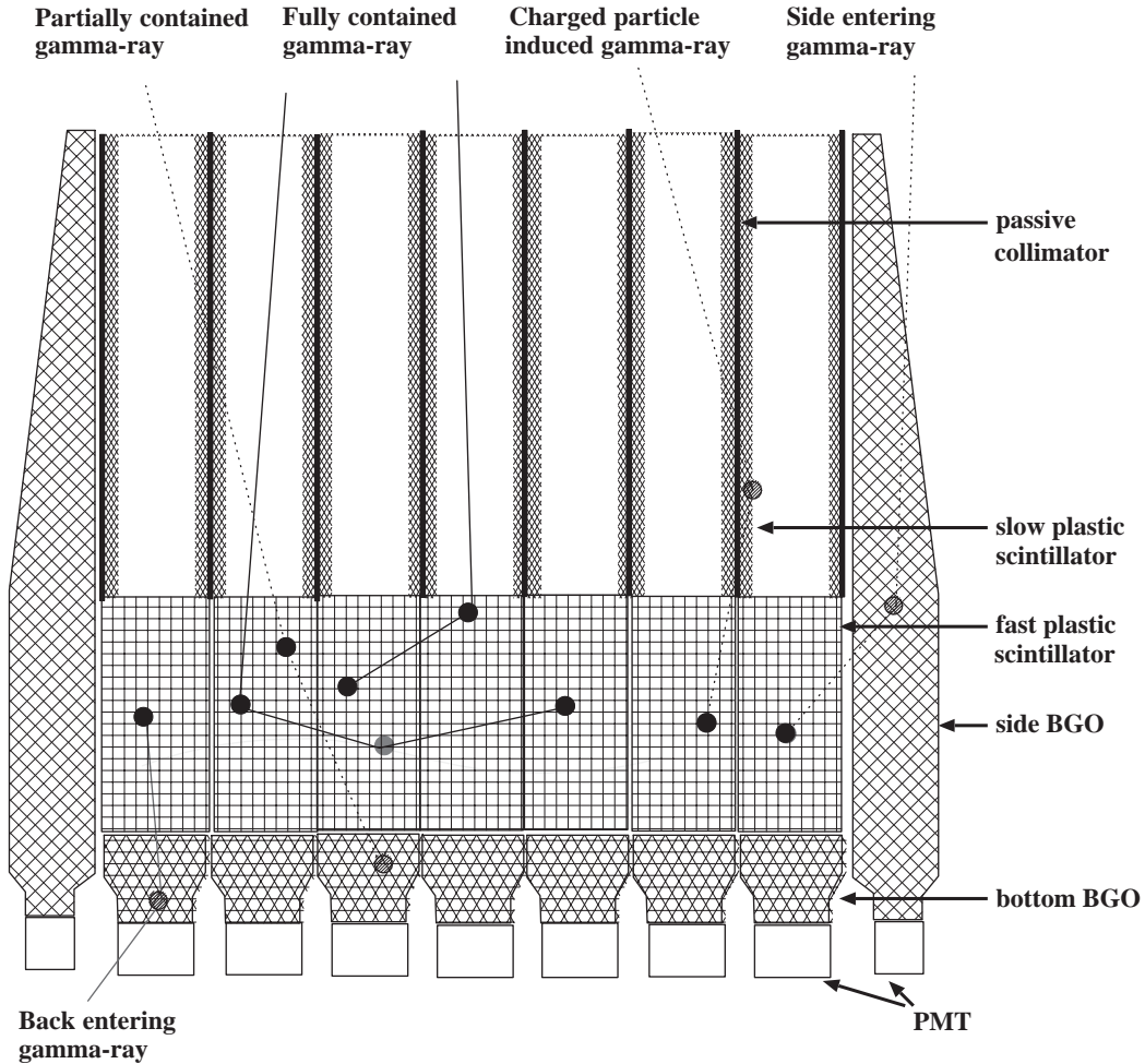
Fig. 1. Conceptual design of PoGO. It consists of an array of well-type phoswich detector units, each made of a fast plastic scintillator, a slow plastic scintillator tube, a thin high-Z metal foil and a bottom BGO. A set of side anti-coincidence detectors made of BGO surrounds the array of phoswich units. In the figure, representative passages of gamma-rays are shown with energy deposition marked by circles. The trigger scheme accepts only the ones marked as “fully contained gamma-ray”.
