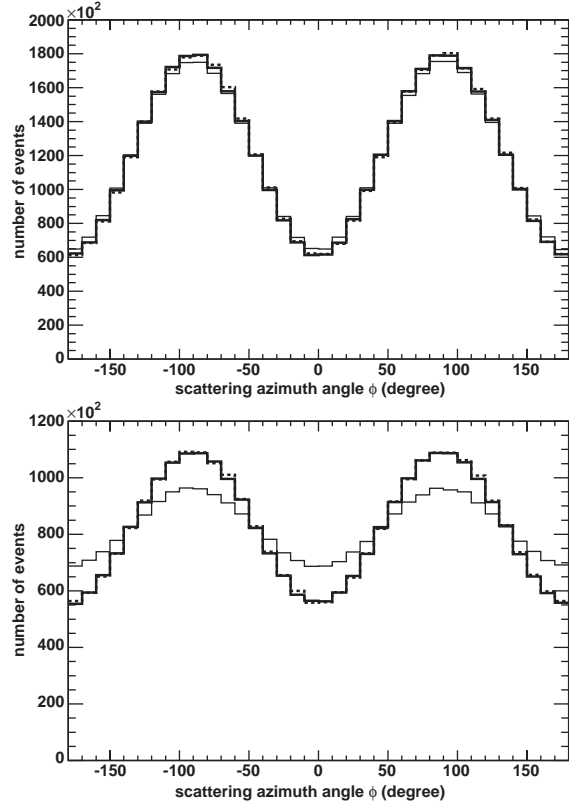
Fig. A3. Azimuthal angle asymmetry of the first (top panel) and the second (bottom panel) Compton scattering for the fully polarized Crab spectrum in 25–200 keV, where the angle is measured from the polarization vector of the incident photon. The distributions of modified Geant4, original Geant4 and EGS4 (all with polarized Compton scattering process) are shown by a thick solid line, a thin solid one and a dotted line, respectively. For Geant4 with our fixes and EGS4 simulation, polarized Rayleigh scattering is also implemented.
